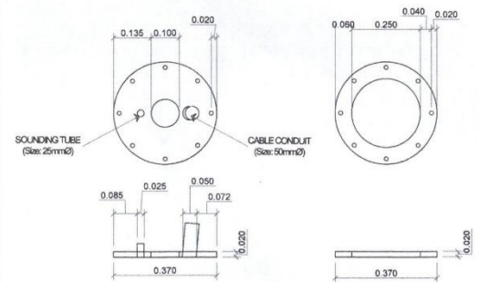
DETAILS OF COVER PLATE AND FLANGE
